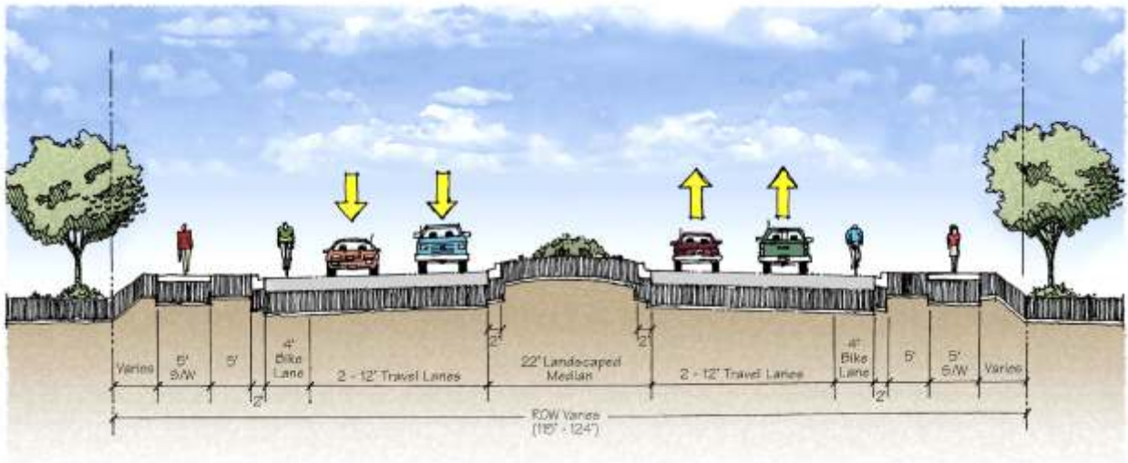
A. From Countryway Boulevard to Montague Street and from Fawn Ridge Boulevard to Sheldon Road
